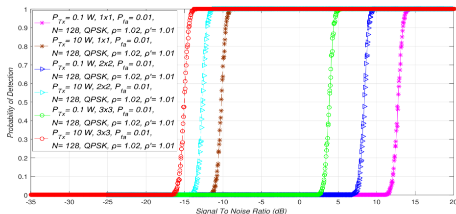
Figure 7. Interdependence between detection probability and SNR for the ED of the signals transmitted with different PU Tx powers in symmetric MIMO transmission systems.
