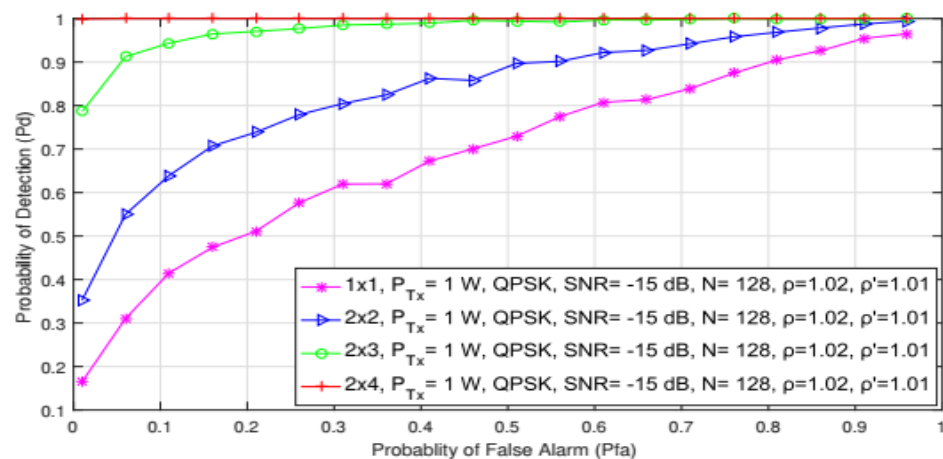
Figure 12. Interdependence between detection and false alarm probabilities for the SISO and symmetric and asymmetric MIMO-OFDM systems.
