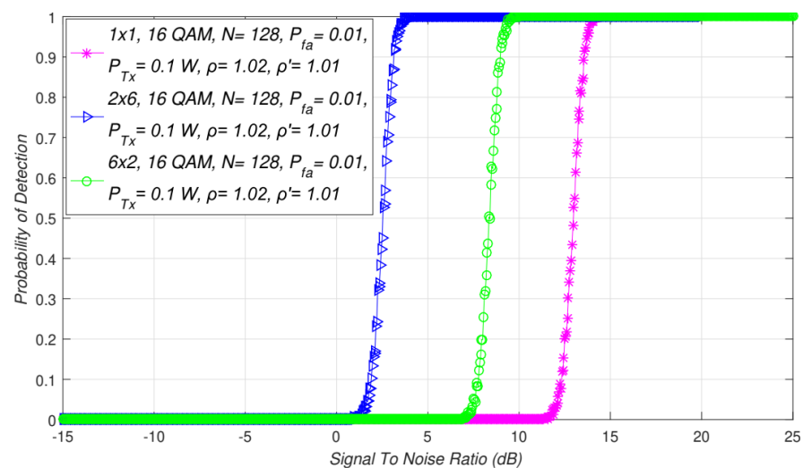
Figure 9. Interdependence between detection probability and SNR for SISO and 2x6 and 6x2 asymmetric MIMO transmission system.
